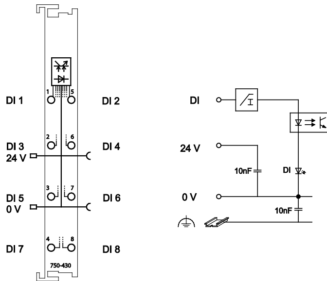
Figure 6: Schematic diagram
